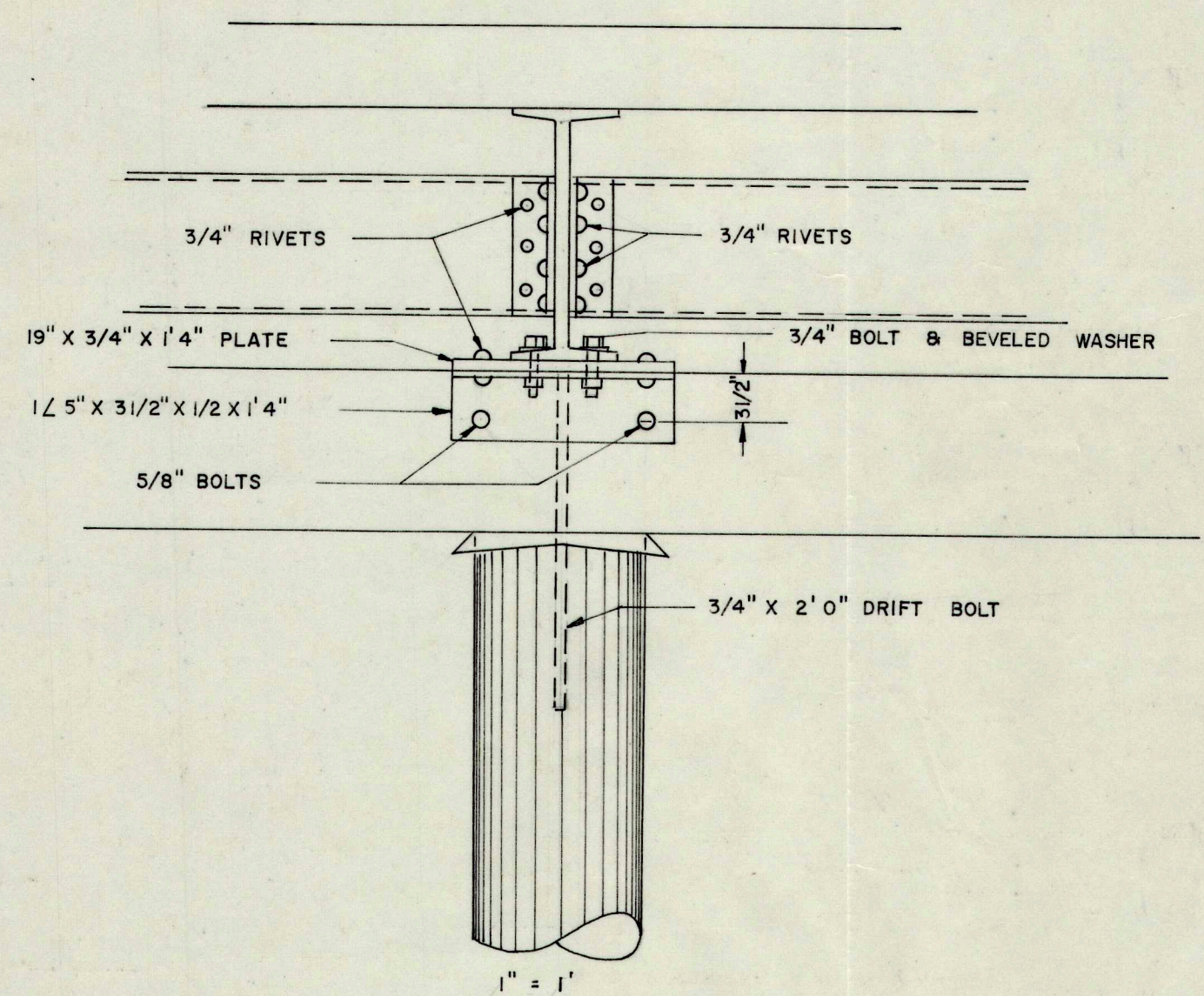
TYPICAL PART CROSS SECTION OF ROADWAY AT BENT
