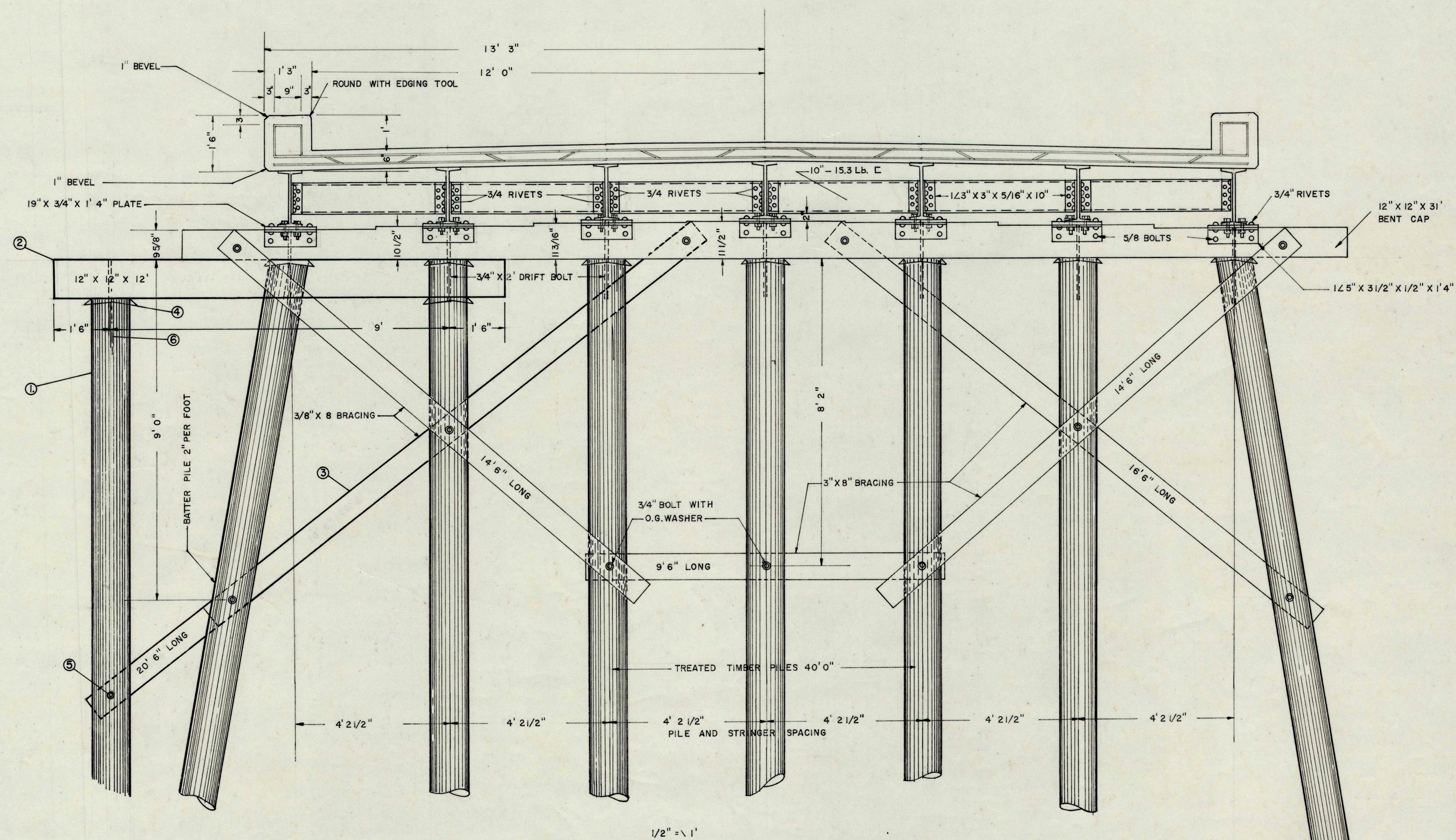
CROSS SECTION OF ROADWAY AT BENT
