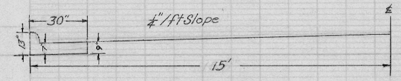
Typical Section for Curb & Gutter
